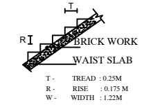
STAIRCASE DETAILS (NOT TO SCALE)
