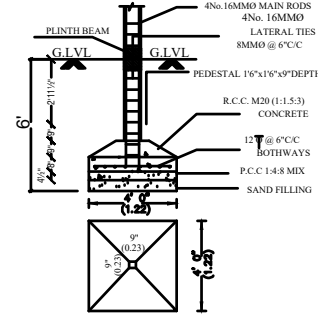
FOUNDATION DETAIL (SCALE: 1/10)
