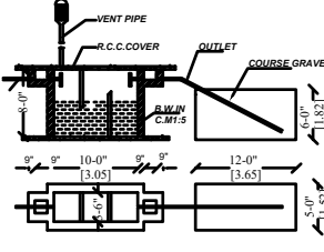
SEPTIC TANK & D-TRENCH DETAILS (NOT TO SCALE)
