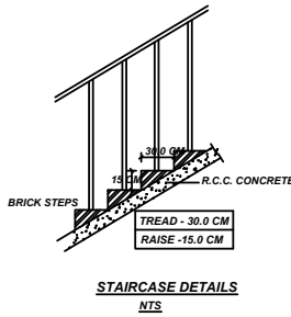
STAIRCASE DETAILS M/E
