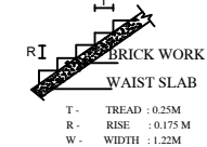
STAIRCASE DETAILS (NOT TO SCALE)
