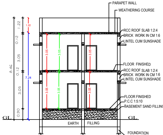
SECTION "J-J"
