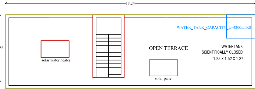
TERRACE FLOOR PLAN
