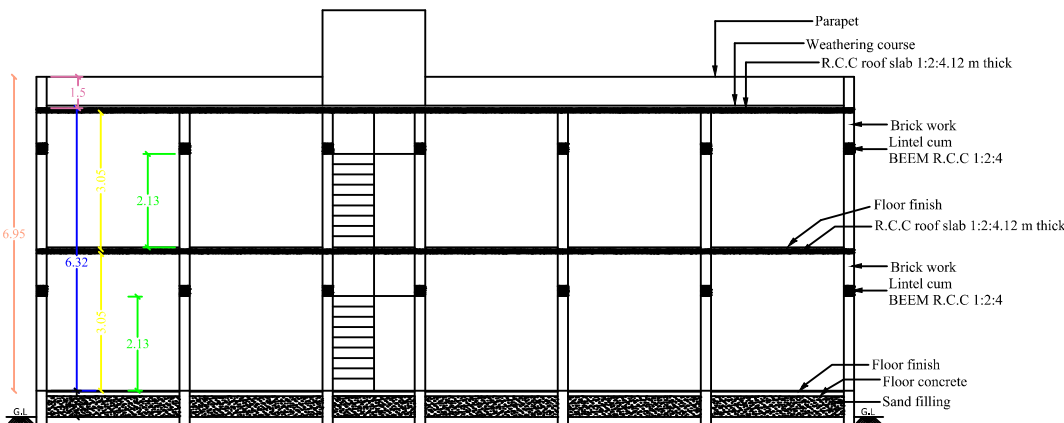
SECTION ON "S - T"
