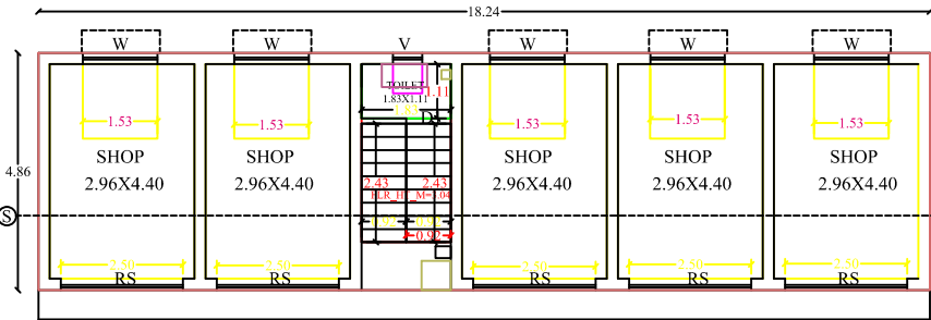
PRO GROUND FLOOR PLAN
