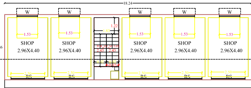
PRO FIRST FLOOR PLAN
