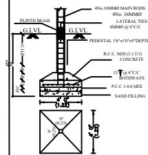
FOUNDATION DETAIL (SCALE: 1/10)
