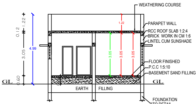
SECTION ON "J-J"
