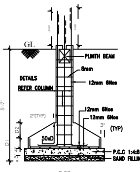
FOUNDATION DETAILS SCALE : 1:50.
