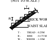
STAIRCASE DETAILS (NOT TO SCALE)
