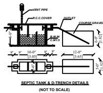
SEPTIC TANK & D-TRENCH DETAILS (NOT TO SCALE)
