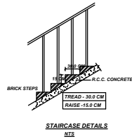
STAIRCASE DETAILS MIS
