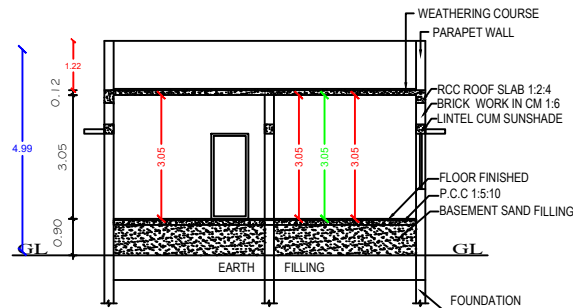
SECTION "J-J"
