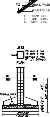
STAIRCASE DETAILS (NOT TO SCALE)
