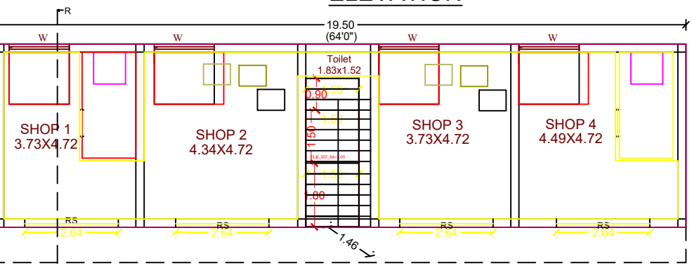
Pro.GROUND FLOOR PLAN
