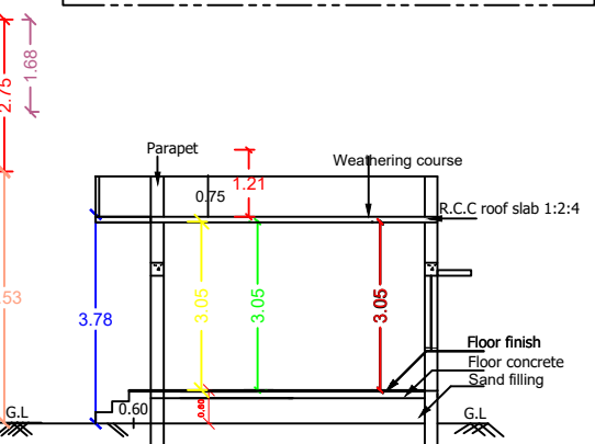
SECTION ON KR
