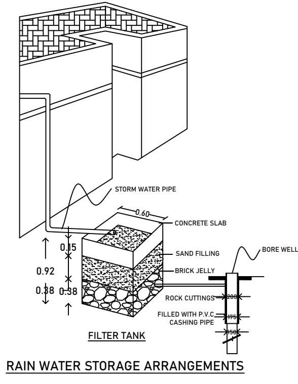
RAIN WATER STORAGE ARRANGEMENTS
