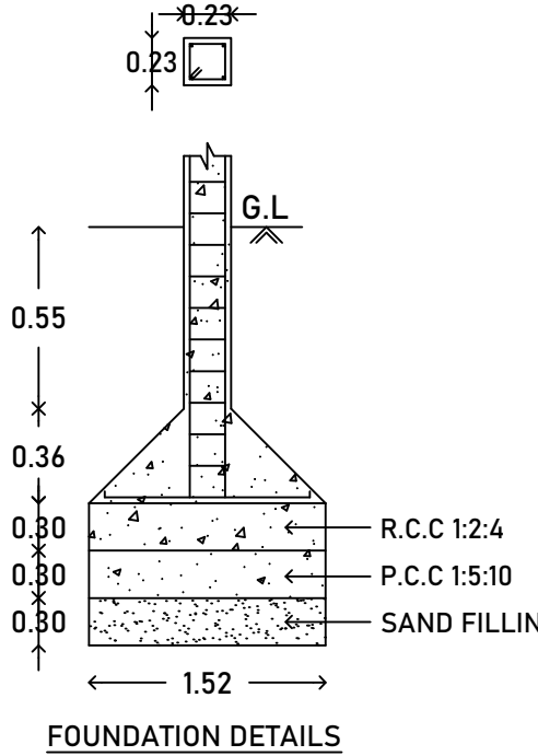
FOUNDATION DETAILS
