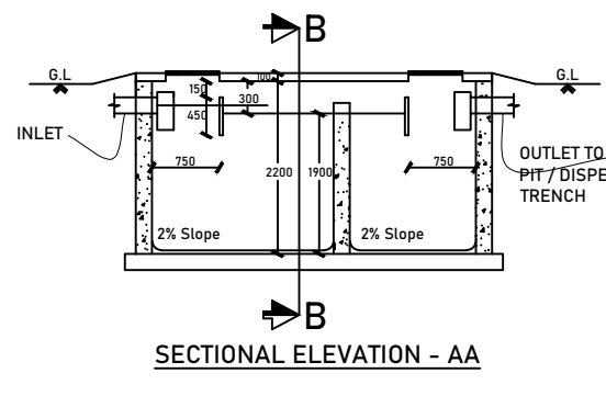
SECTIONAL ELEVATION - AA
