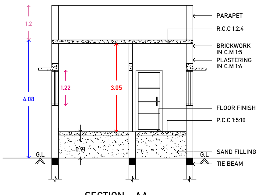
SECTION - AA
