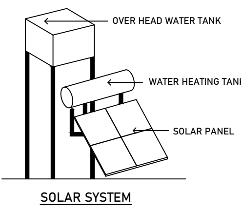
SOLAR SYSTEM
