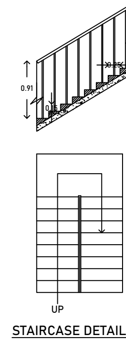
STAIRCASE DETAILS
