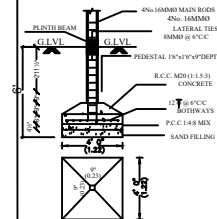
FOUNDATION DETAIL (SCALE: 1/10)
