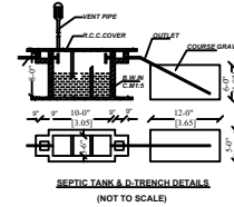
SEPTIC TANK & D-TRENCH DETAILS (NOT TO SCALE)
