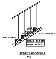
STAIRCASE DETAILS MIS
