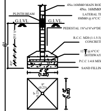
FOUNDATION DETAIL (SCALE: 1/10)
