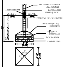
FOUNDATION DETAIL
