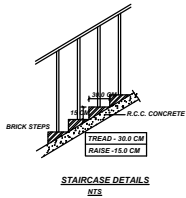
STAIRCASE DETAILS MIS
