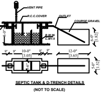
SEPTIC TANK & D-TRENCH DETAILS (NOT TO SCALE)
