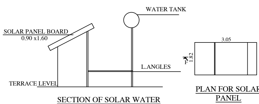
SECTION OF SOLAR WATER HEATER
