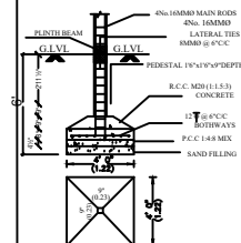
FOUNDATION DETAIL
