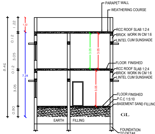
SECTION "J-J"
