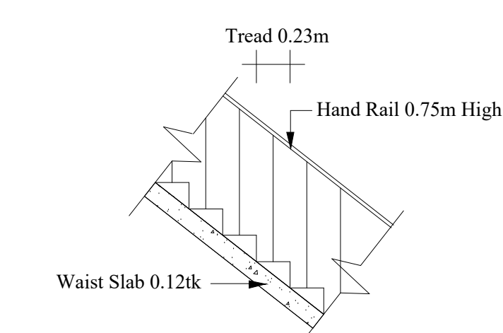
STAIR DETAILS SCALE : NOT TO SCALE
