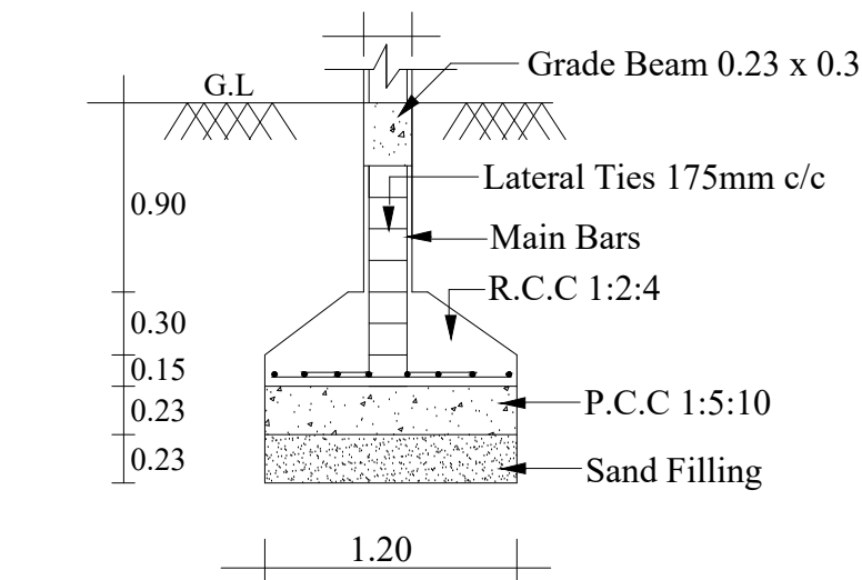
FOOTING DETAILS SCALE : NOT TO SCALE
