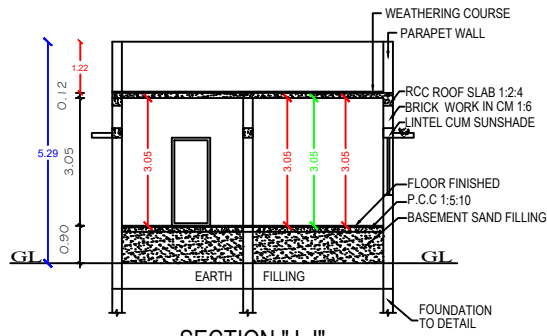
SECTION "J-J"
