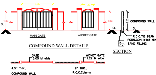
COMPOUND WALL PLAN
