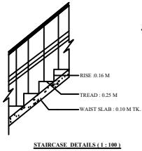
STAIRCASE DETAILS (1 : 100)
