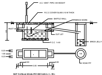
SEW TANK & SOAK PIT DETAILS (1 : 20)
