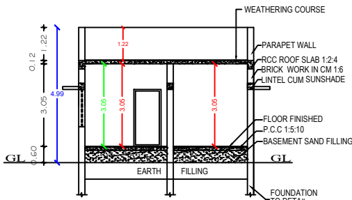
SECTION "J-J"
