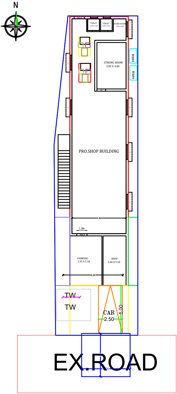
SITE PLAN
