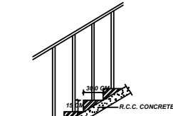
STAIRCASE DETAILS
