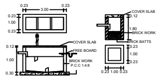
DETAILS OF SEPTIC TANK AND SOAK PIT (NOT TO SCALE)
