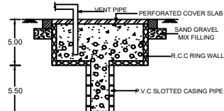
DETAILS OF RAINWATER HARVESTING PIT (NOT TO SCALE)
