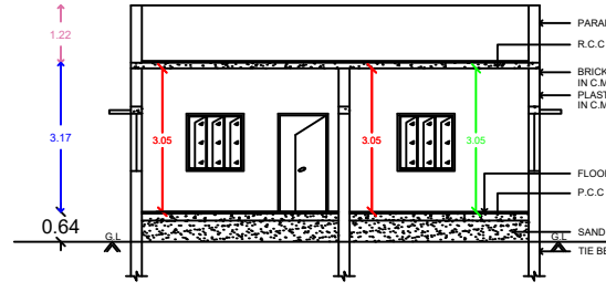
SECTION RS
