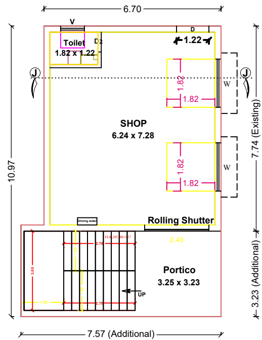
EX & ADD.GROUND FLOOR PLAN
