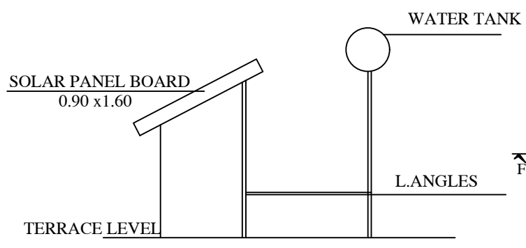
SECTION OF SOLAR WATER HEATER
