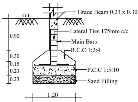
FOOTING DETAILS SCALE : NOT TO SCALE
