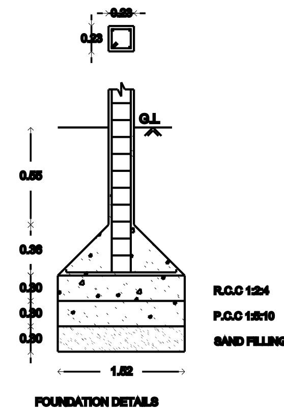
FOUNDATION DETAILS
