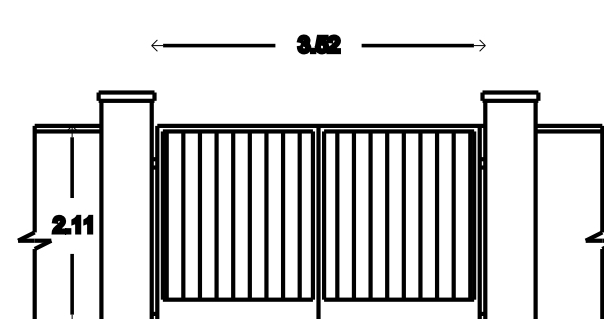
MAIN GATE
