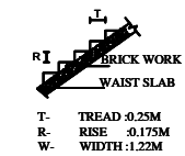
STAIRCASE DETAILS (NOT TO SCALE)
