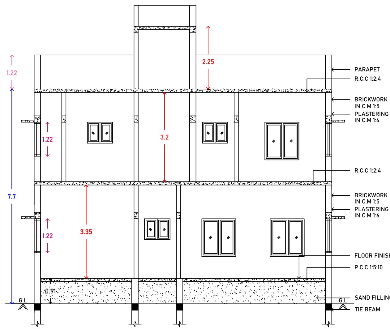
SECTION - AA
