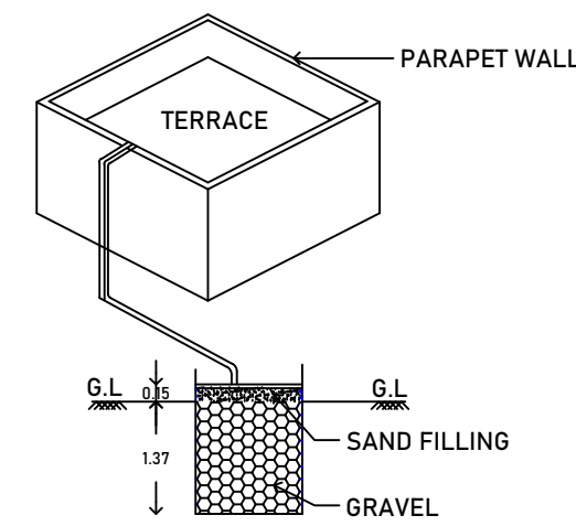
COLLECTION SUMP FOR HARVESTING FOR TERRACE
