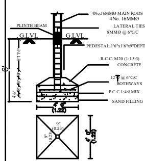
FOUNDATION DETAIL
