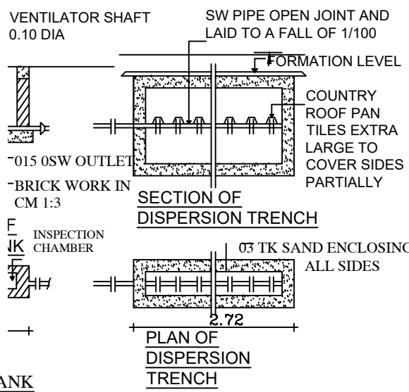
PLAN OF DISPERSION TRENCH
