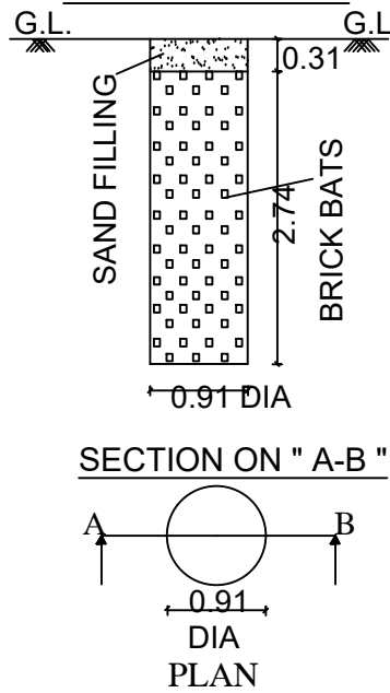
DETAILED PLAN OF RAINWATER PERCUATION AND COLLECTION PIT
