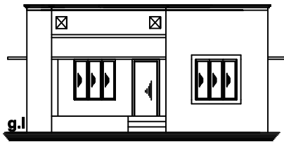
Building Front Elevation
