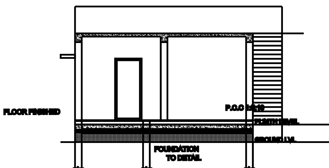
SECTION AB
