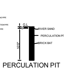
PERCOLATION PIT
