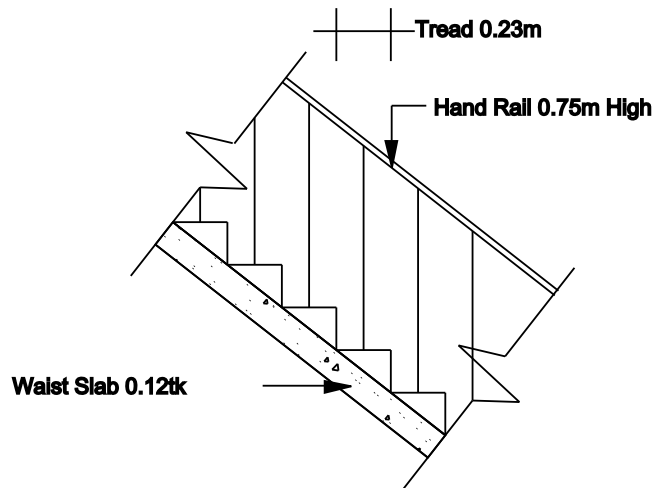
STAIR DETAILS SCALE : 1:50
