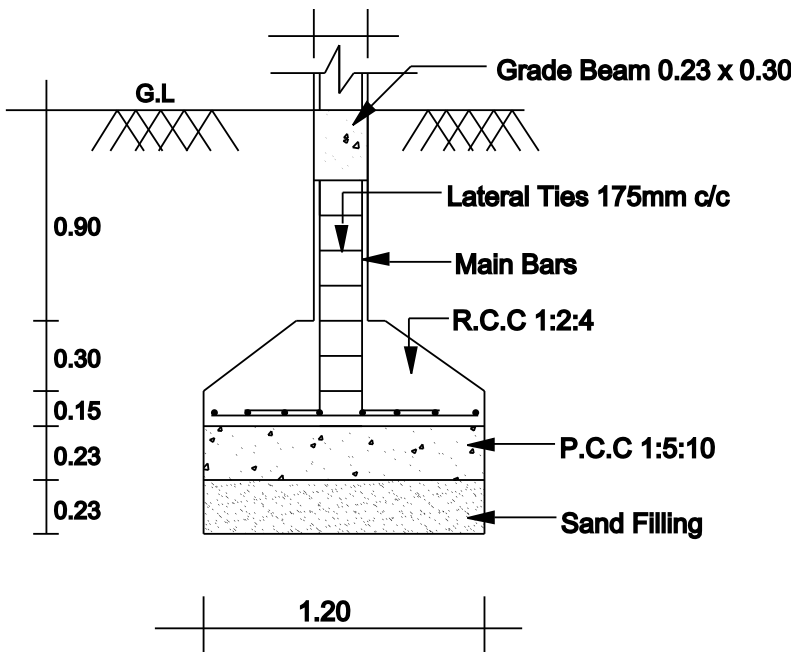
FOOTING DETAILS SCALE : NOT TO SCALE
