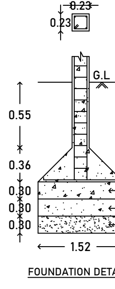
FOUNDATION DETAILS
