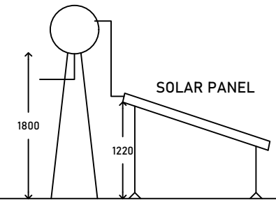
SIDE ELEVATION (NOT TO SCALE)
