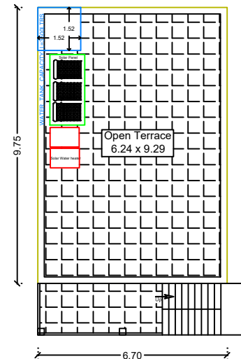
R PLAN
