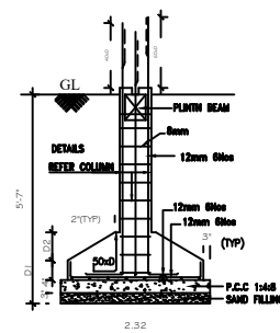
FOUNDATION DETAILS
