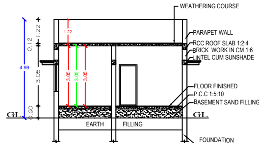
SECTION ON "J-J"
