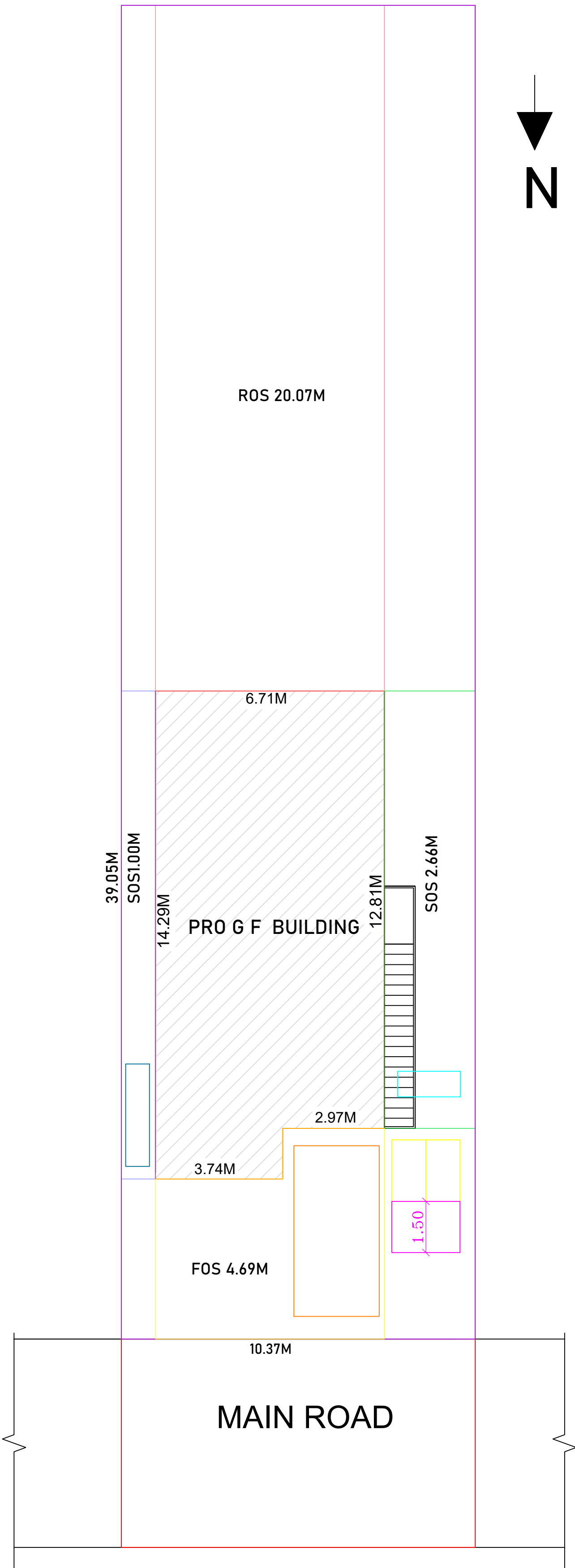
SITE PLAN
