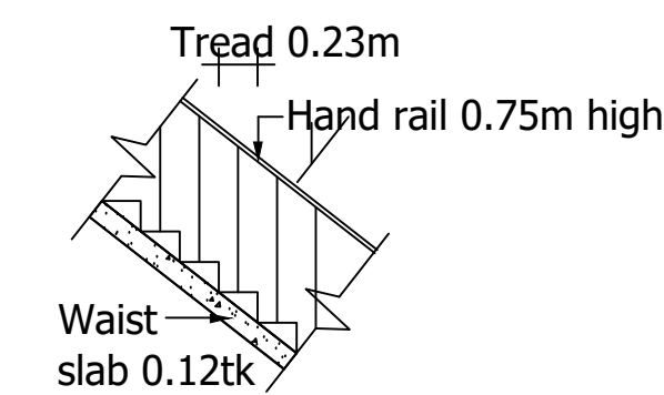
STAIR DETAILS
