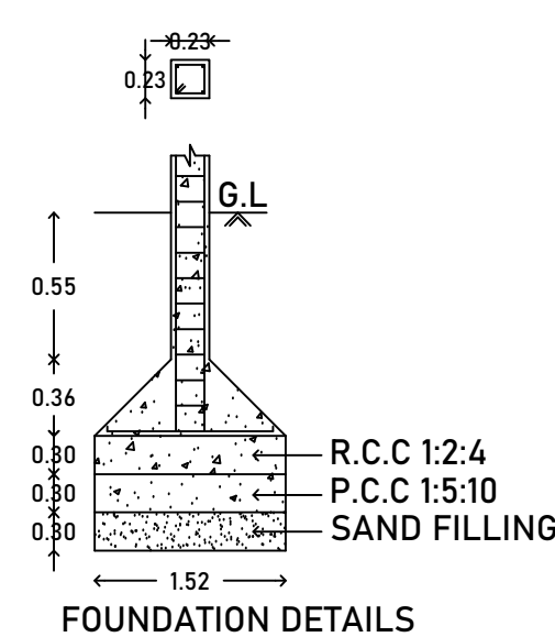
FOUNDATION DETAILS
