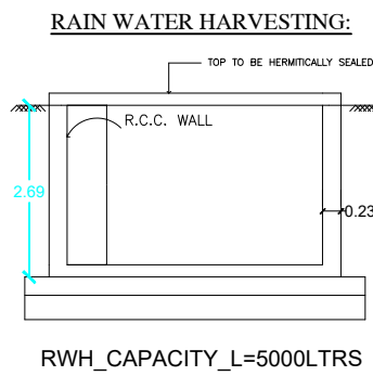
RWH_CAPACITY_L=5000LTRS RWH_CAPACITY_L=5000LTRS
