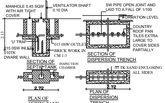
DETAILED DRAWING FOR SEPTIC TANK WITH DISPERSION TRENCH 225 GALLONS CAPACITY OF 1000 LITERS
