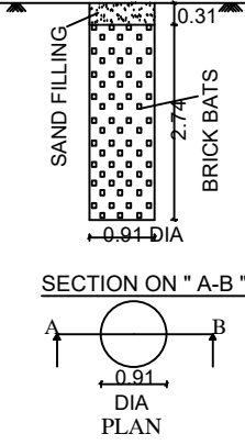
DETAILED PLAN OF RAINWATER PERCOLATION AND COLLECTION PIT
