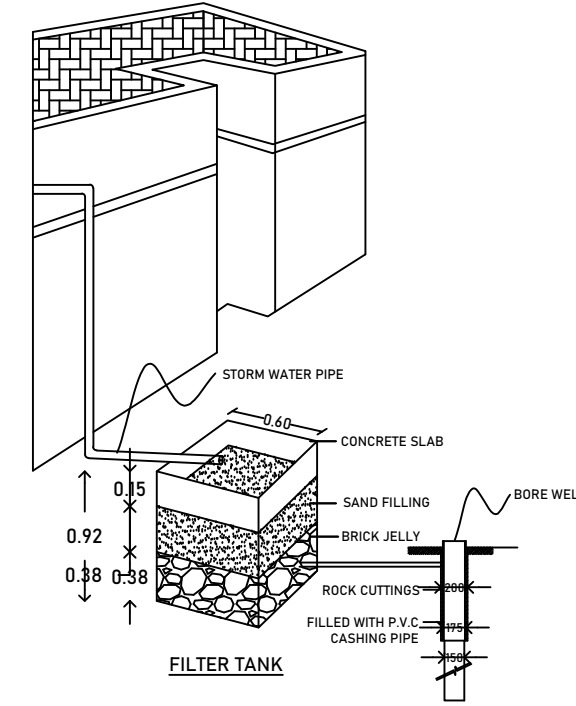
RAIN WATER STORAGE ARRANGEMENTS
