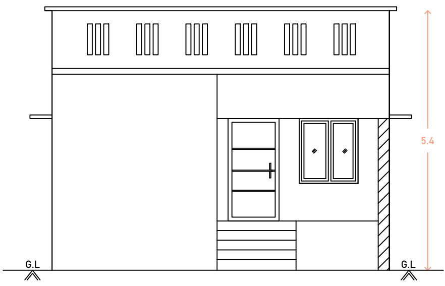
FRONT ELEVATION
