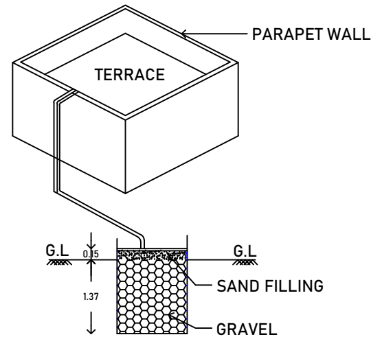
COLLECTION SUMP FOR HARVESTING FOR TERRACE
