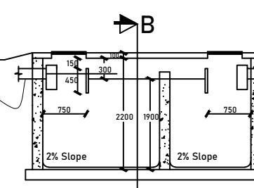
SECTIONAL ELEVATION - AA
