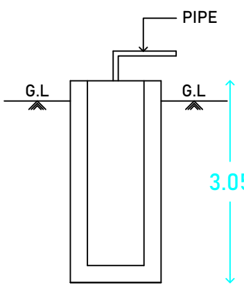
DETAILS OF RAINWATER COLLECTION TANK
