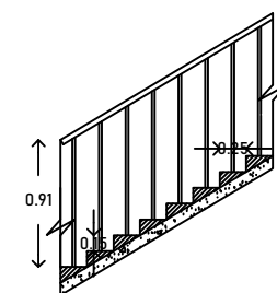
STAIRCASE DETAILS
