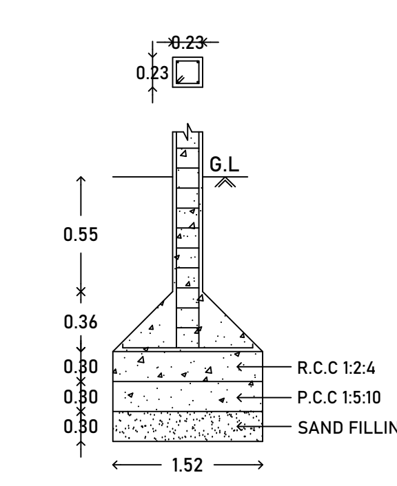
FOUNDATION DETAILS
