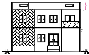
FRONT ELEVATION
