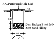
RAIN WATER HARVEST PIT SCALE : NOT TO SCALE
