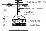
FOOTING DETAILS SCALE : NOT TO SCALE
