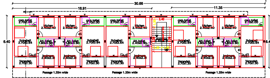
PRO.F.F RESIDENTIAL BUILDING PLAN (five numbers of colony Residential building)
