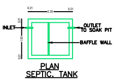
PLAN SEPTIC TANK
