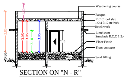
SECTION ON "N - R"
